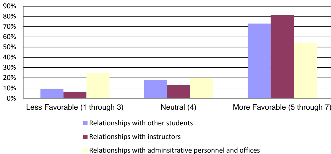
Figure 1: Relationships
